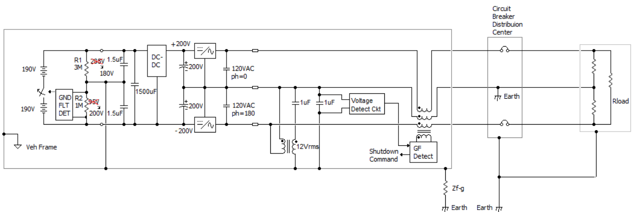
Figure 10 – Supplementary Grounded Neutral Protection
