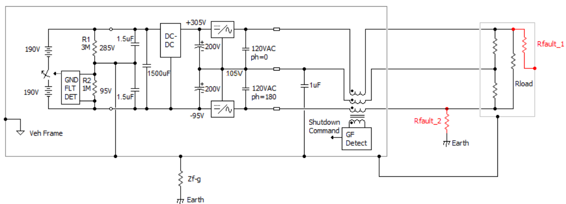
Figure 7 – AC Ground Fault Detection Circuit with Reference Impedance Neutral to Vehicle Ground
