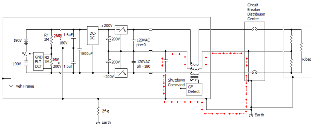
Figure 9 – Export Power with Grounded Remote Neutral
