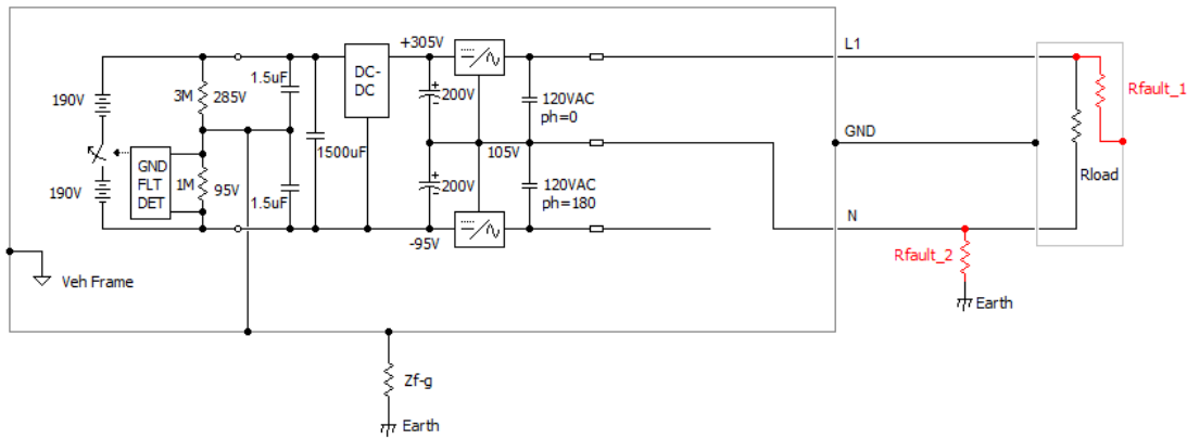
Figure 4 – Export 120VAC Power
