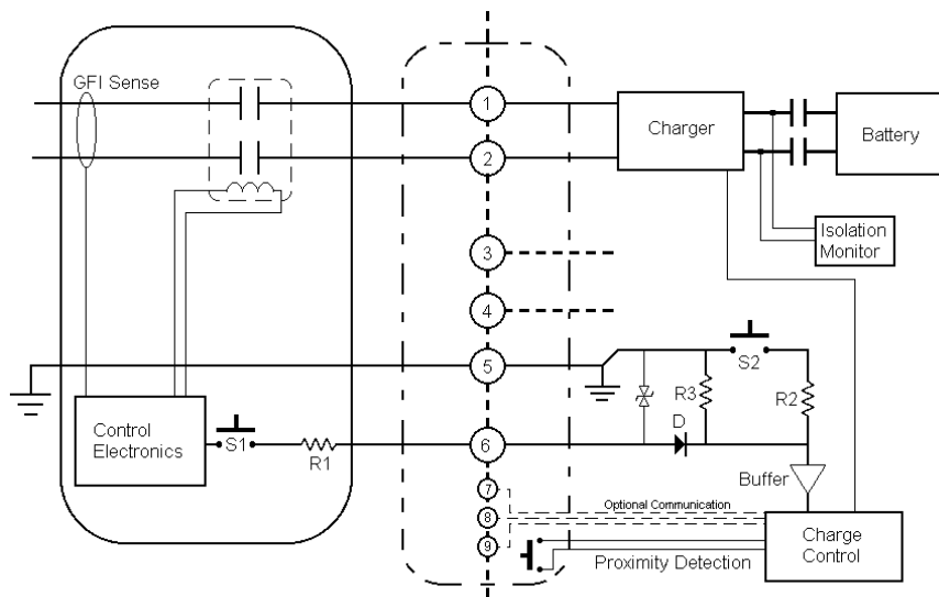
Figure 11 – AC Level 2 EVSE System Diagram
