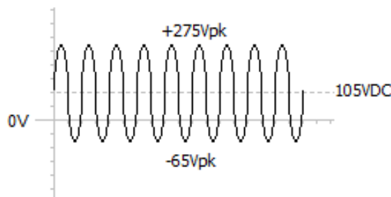
Figure 5 – Export Output voltage with respect to Earth Ground – Ungrounded Neutral terminal
