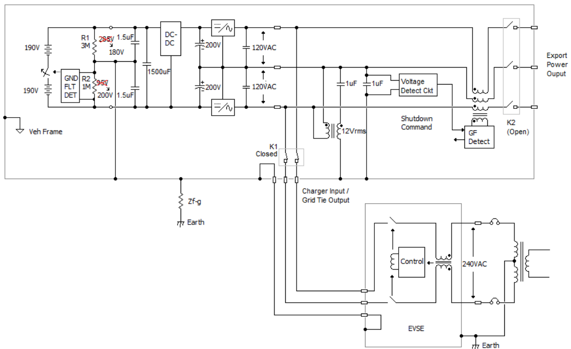
Figure 12 – Grid-tie Power Mode
